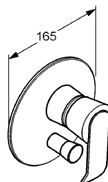
Dimensional drawing
