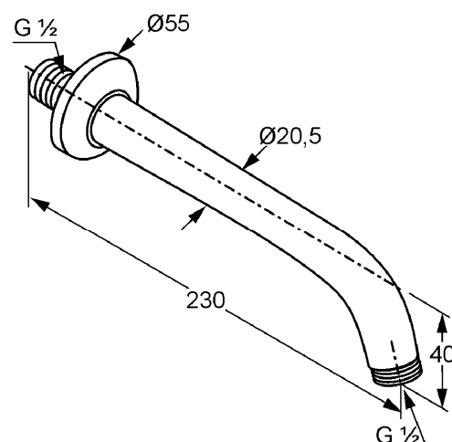
Dimensional drawing
