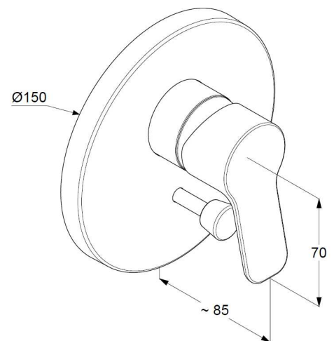
Dimensional drawing
