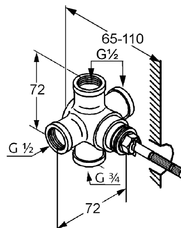
Dimensional drawing II
