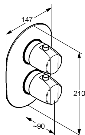
Dimensional drawing I
