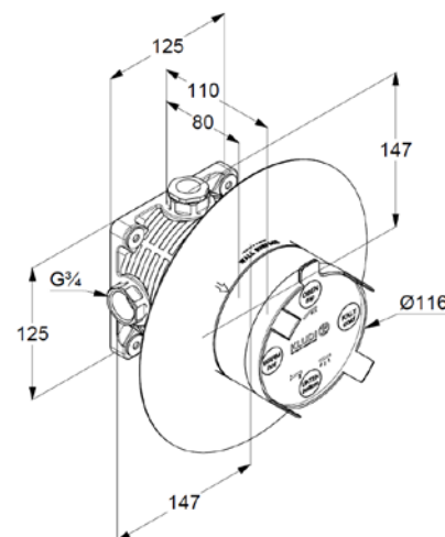
Dimensional drawing
